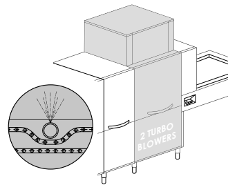
DRF99MB1 + 900mm 16.1 kW Stage dryers with blowers and lower belt
